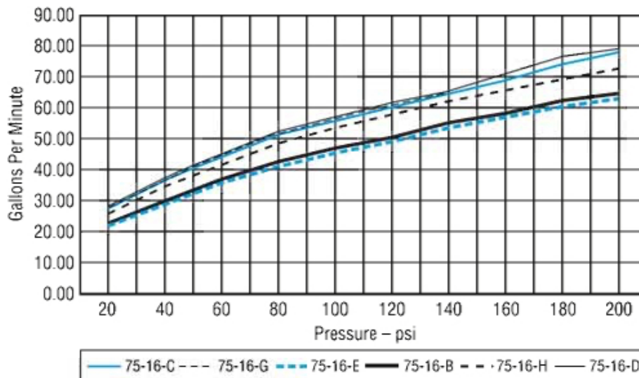
NOMINAL PRESSURE FLOW CURVES
