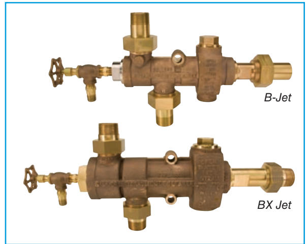
All Hydraulic Jets have the capability to siphon chemical or detergent if needed for maximum cleaning efficiency.
